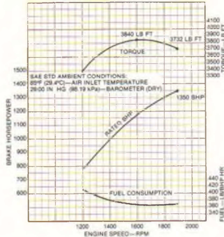
PRELIMINARY ENGINE PERFORMANCE MODEL 12V-149T1 WITH 195 INJECTORS
