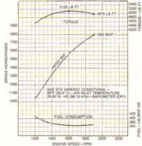
PRELIMINARY ENGINE PERFORMANCE MODEL 16V-149T1 WITH 195 INJECTORS
