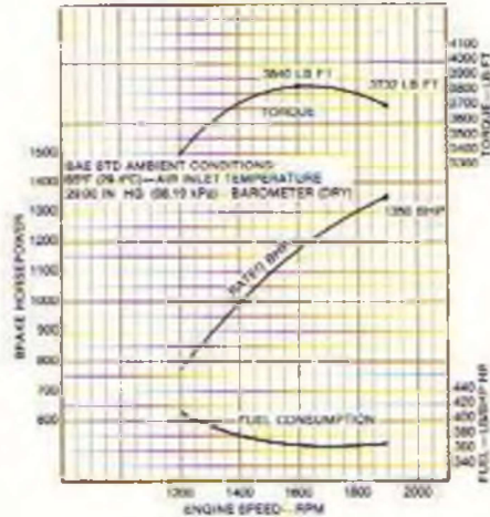
PRELIMINARY ENGINE PERFORMANCE MODEL 12V-146TI WITH 195 INJECTORS
