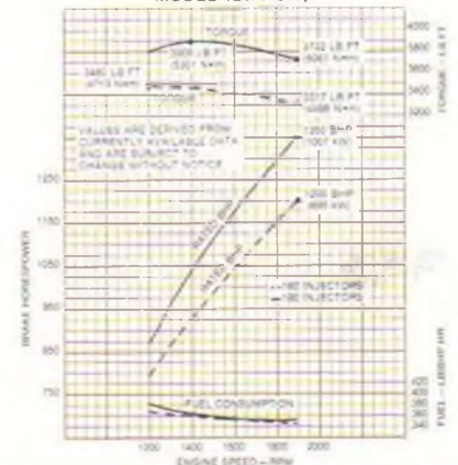
BASIC ENGINE PERFORMANCE MODEL 12V-149TI†
