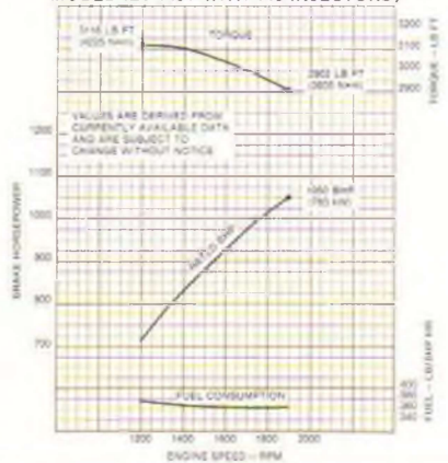
BASIC ENGINE PERFORMANCE MODEL 12V-149T WITH 145 INJECTORS†
