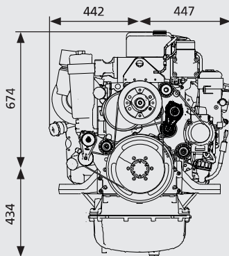
All dimensions in mm
